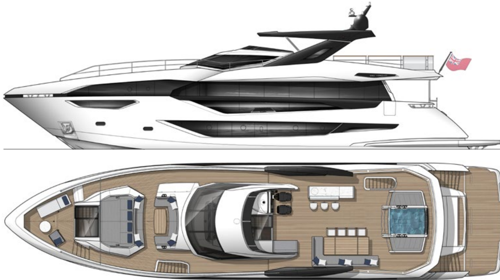
PROFILE AND FLYBRIDGE
