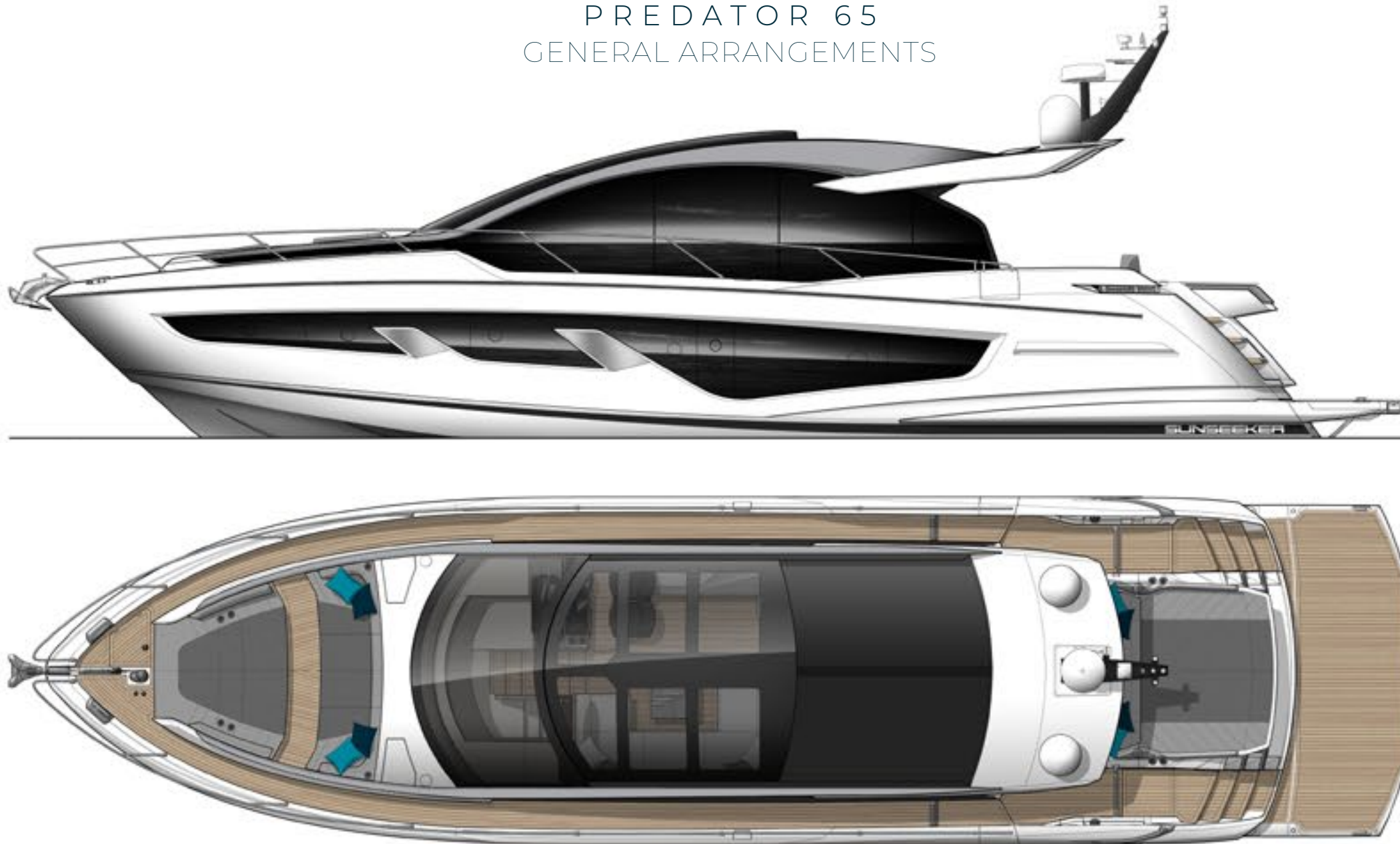
PROFILE AND EXTERIOR PLAN
