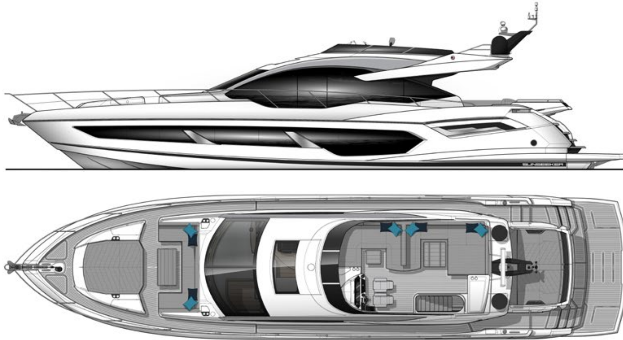
PROFILE AND FLYBRIDGE
