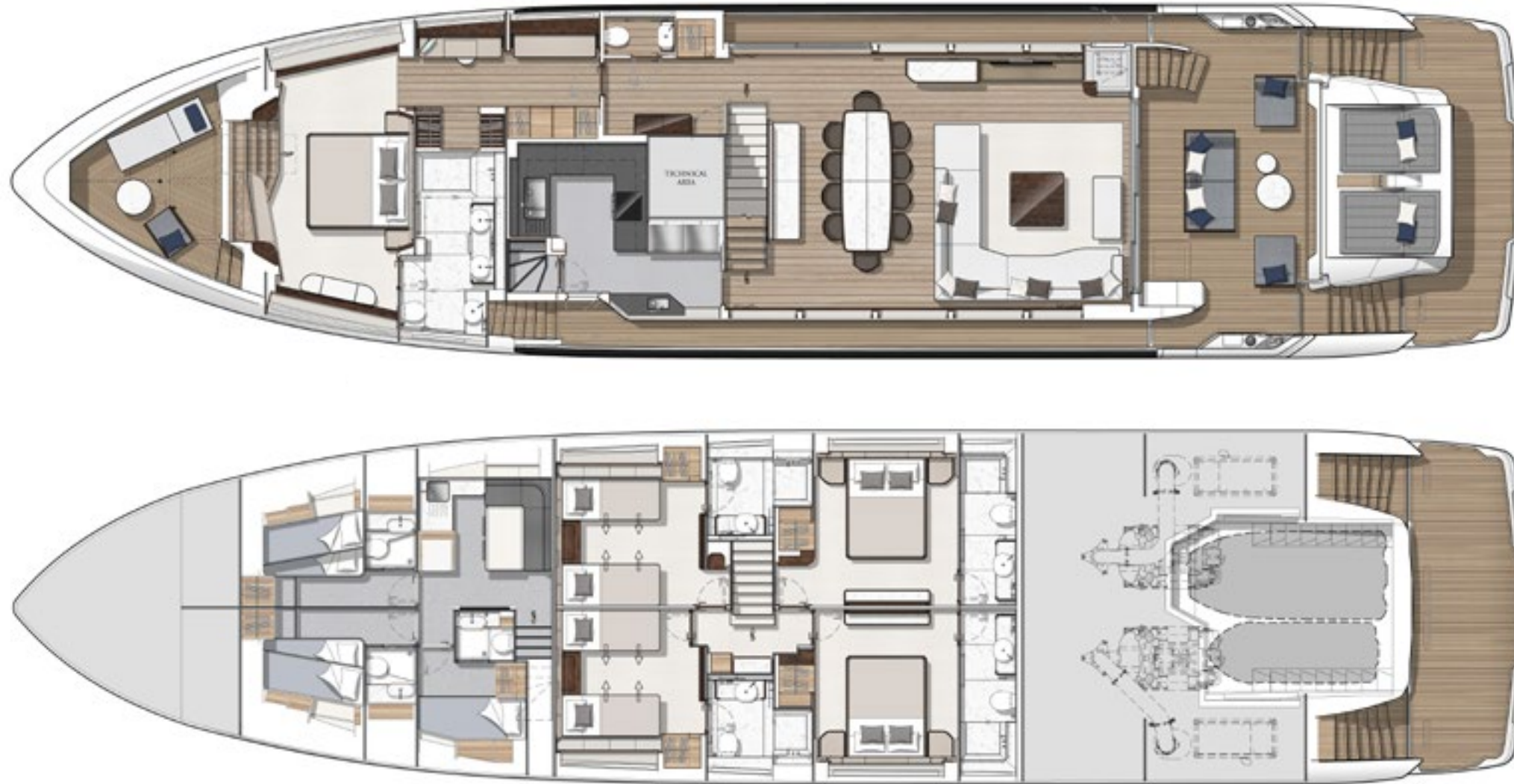
MAIN AND LOWER DECK
