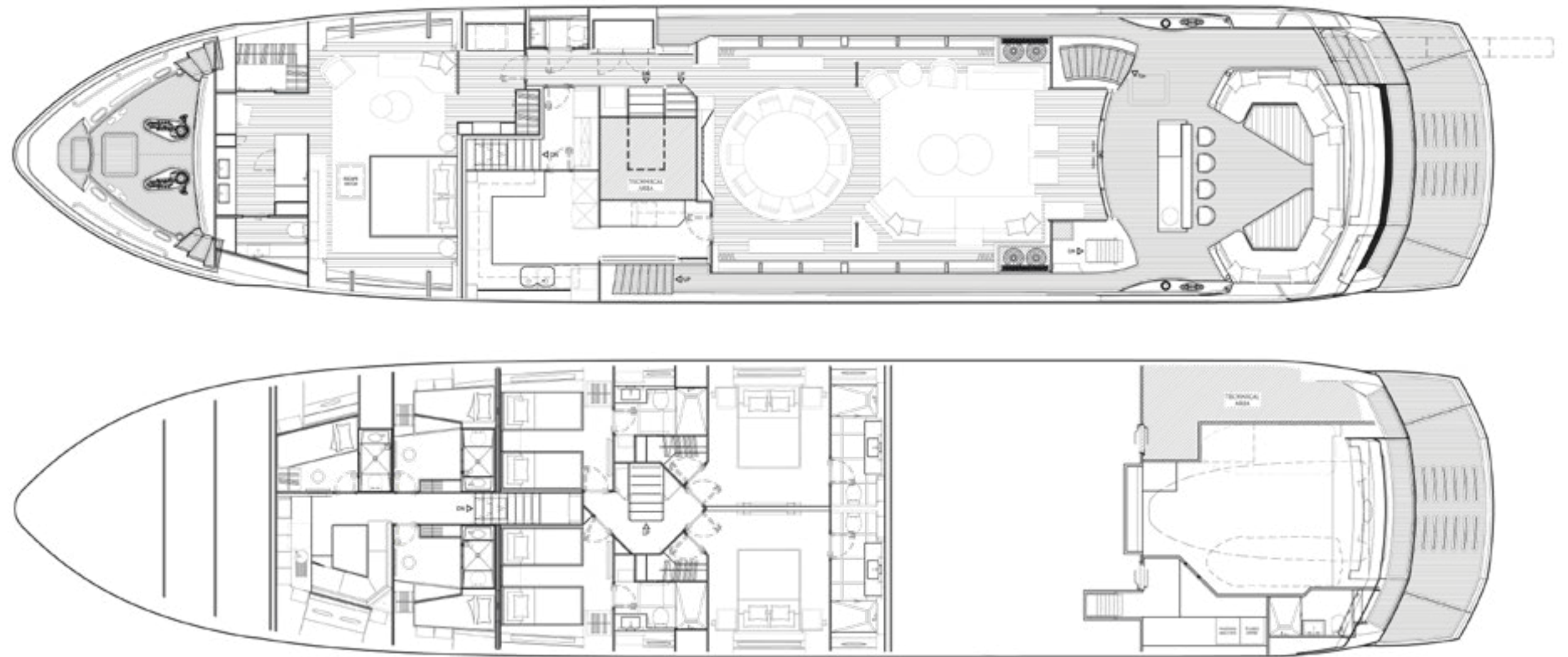
MAIN AND LOWER DECK
