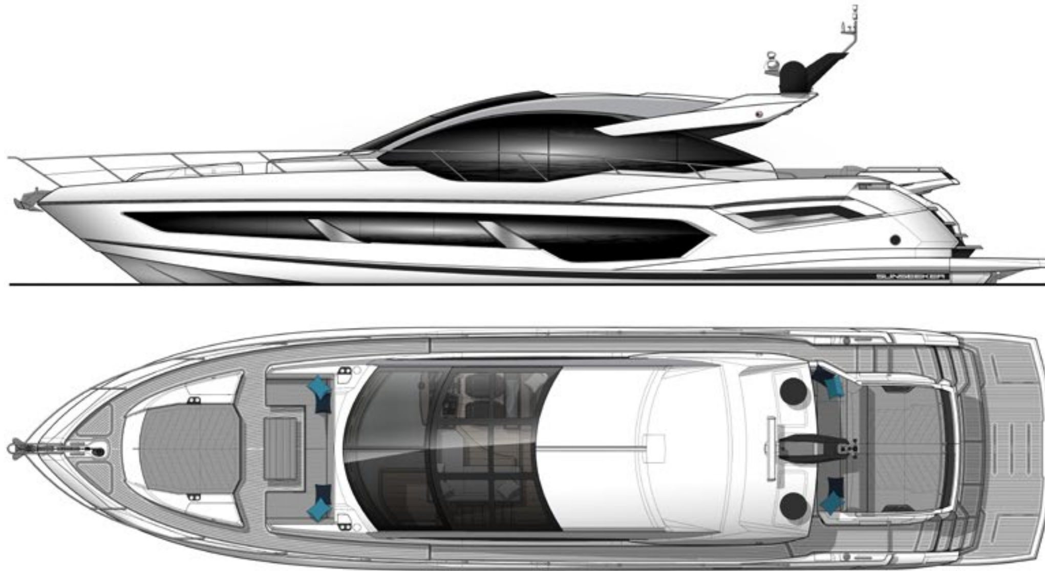
PROFILE AND EXTERIOR PLAN
