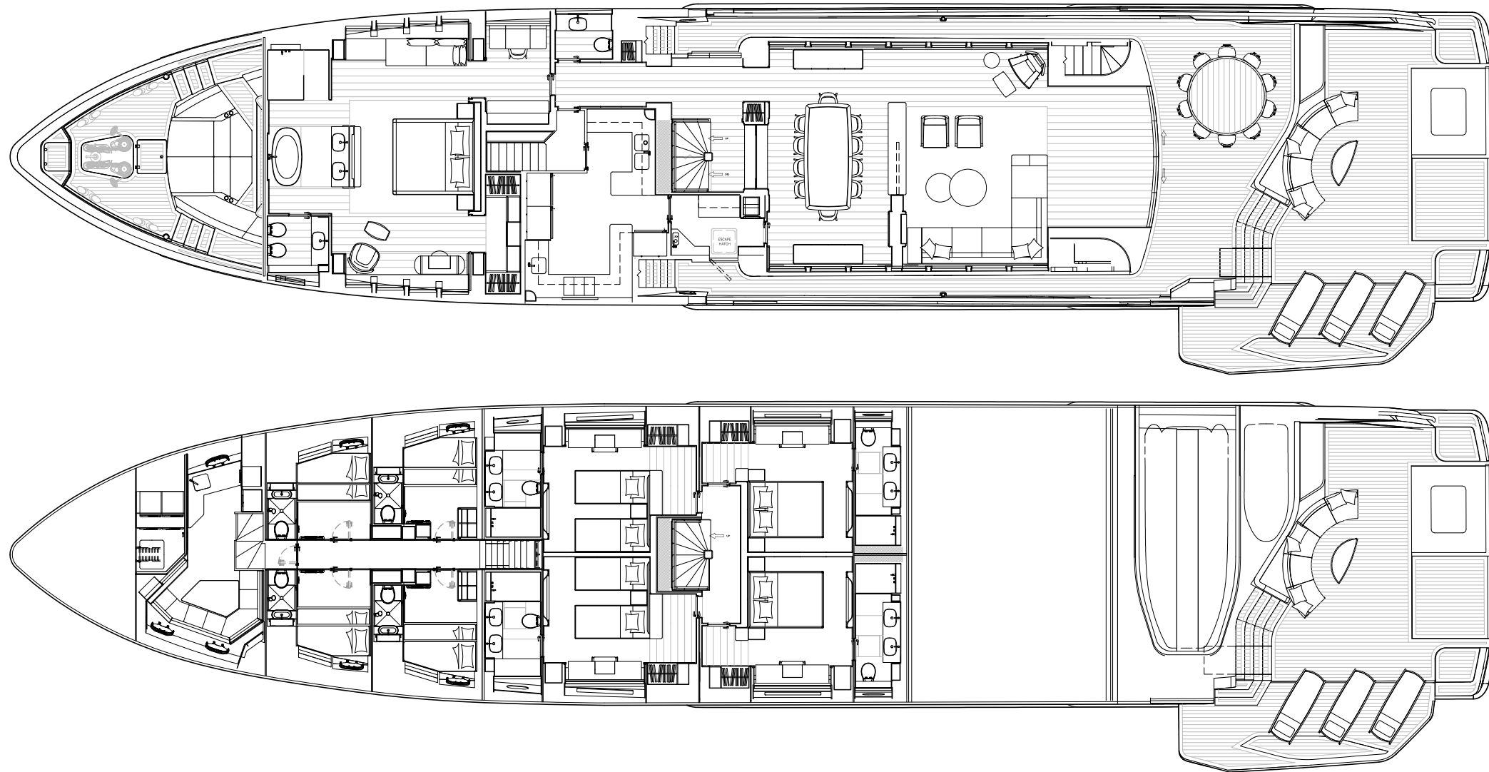
MAIN AND LOWER DECK
